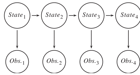
Figure 10: Structure of a hidden Markov model.
