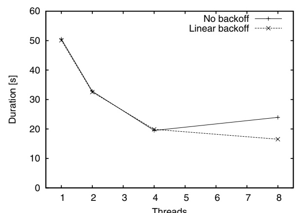
Figure 11. Execution time of backoff vs. no backoff (in SwissTM) in the STAMP intruder application
